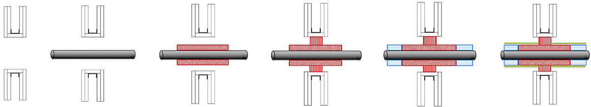
Figure 38 Sequence of installation
