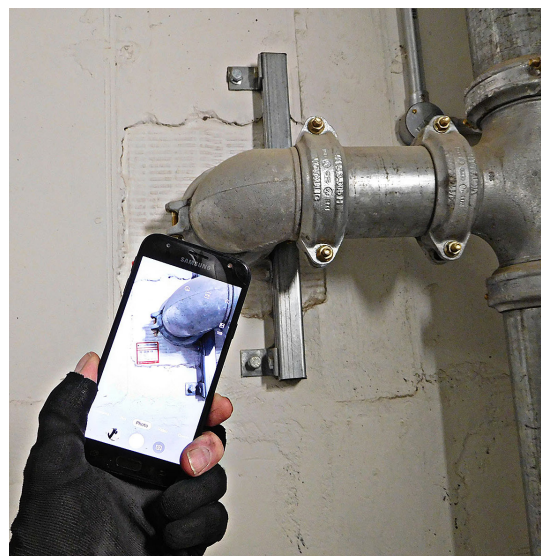
Figure 33 Electronic recording of a penetration seal installation
