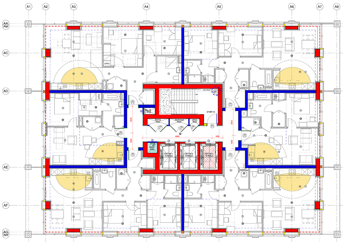
Figure 3 Typical fire strategy plan with coloured compartment walls illustrating the fire ratings required
