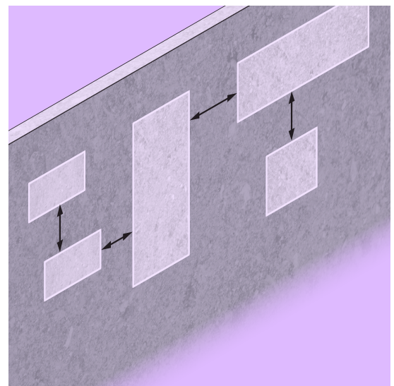
Figure 12 Proximity of penetration seals
